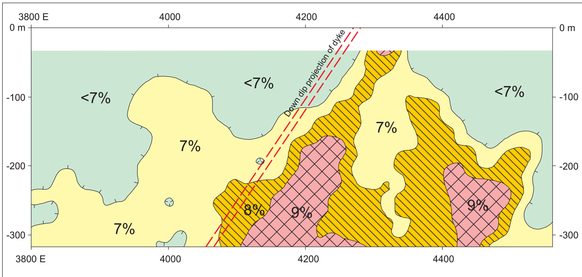
Figure 5. Chargeability pseudosection, line 410, zone III.
